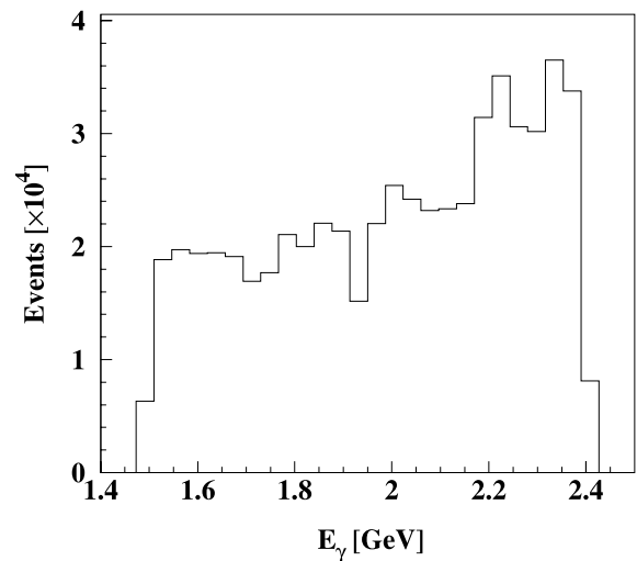
Fig. 4. The tagged photon energy spectrum
